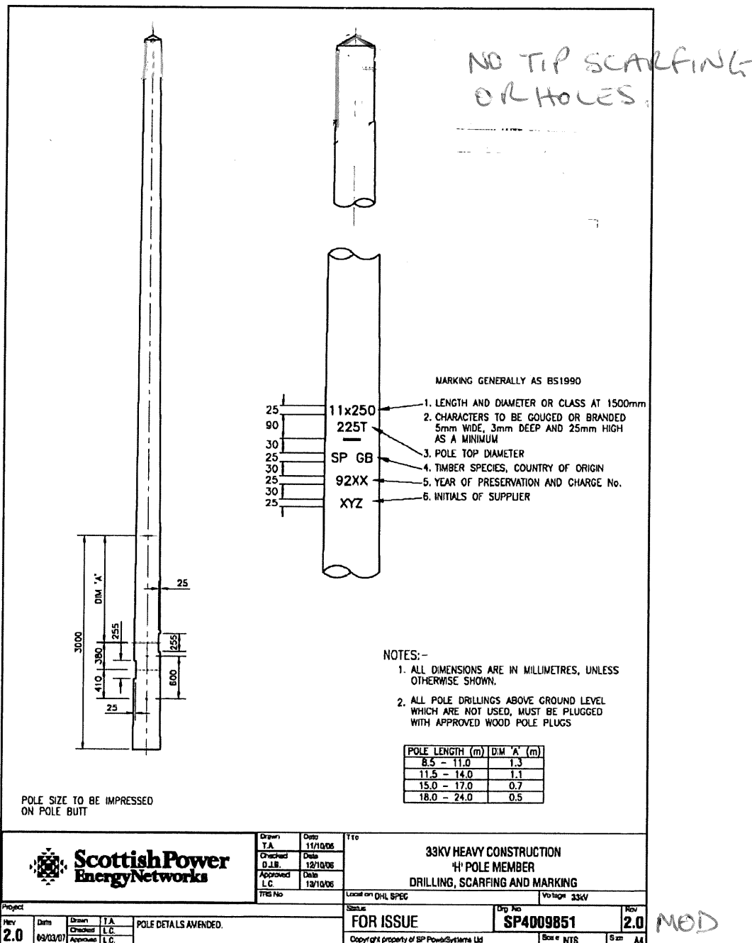
Figure 6 33kV Heavy Construction H Pole Member Drilling, Scarfing and Marking
